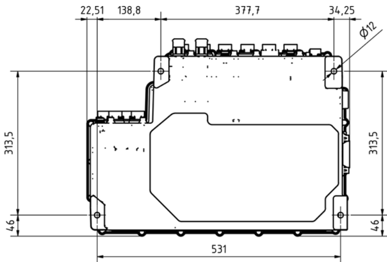
Figure 4: View from below with hole pattern
