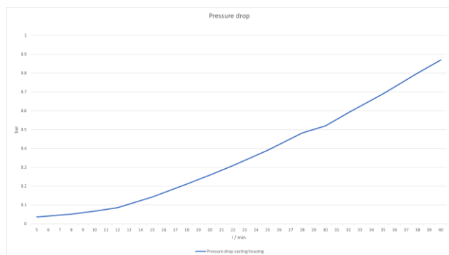
Figure 1: Pressure drop in the cooling system at a coolant temperature of 20°C
