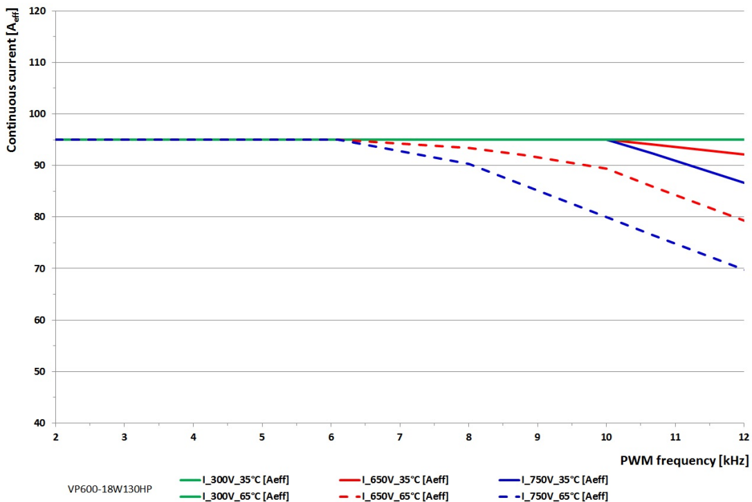
Continuous current depends on voltage, PWM frequency and cooling water temperature
