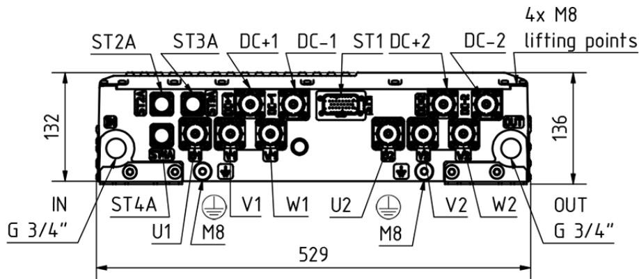
Figure 2: Front view, position of the connections
