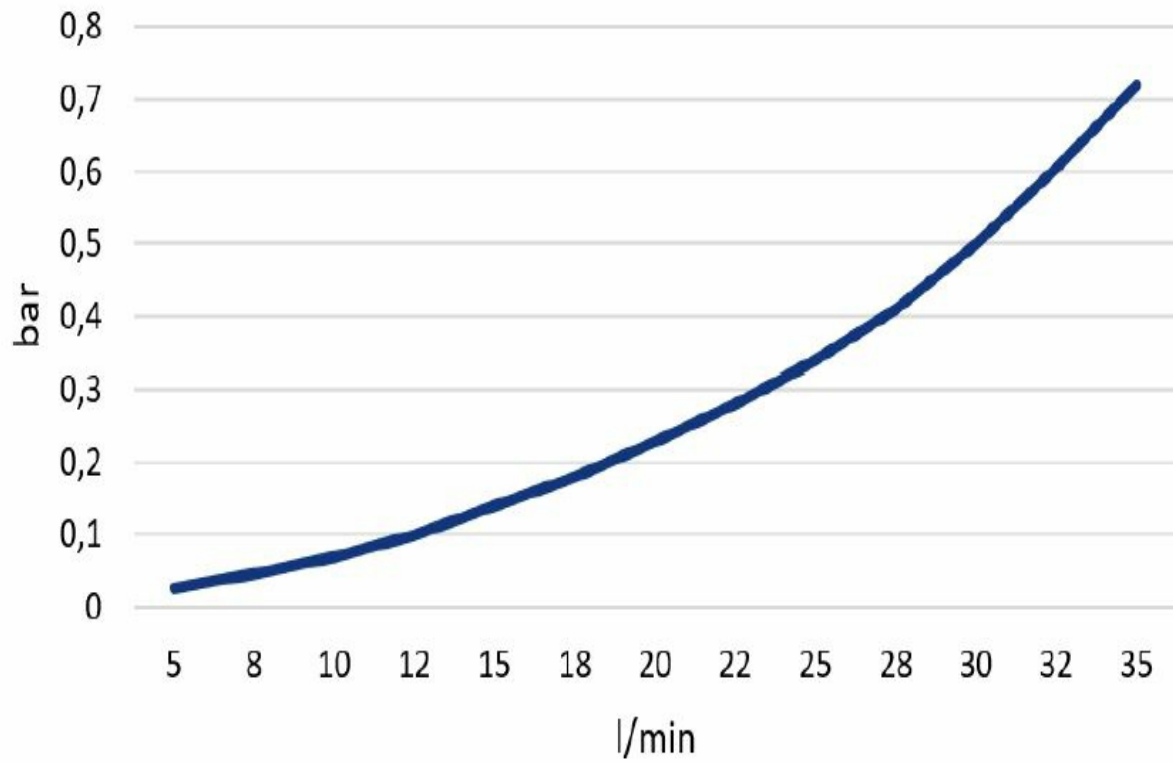
Illustration: pressure loss vs coolant flow
