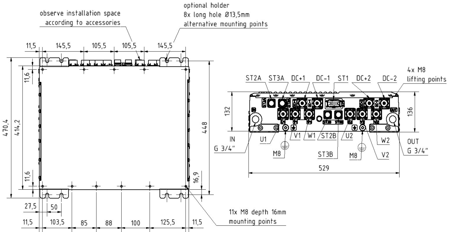
Illustration: Dimensions
