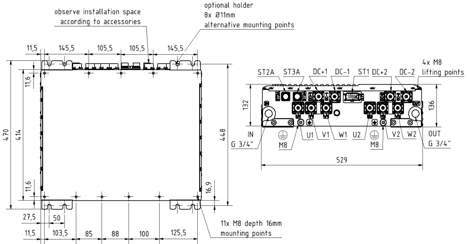
Illustration: Dimensions
